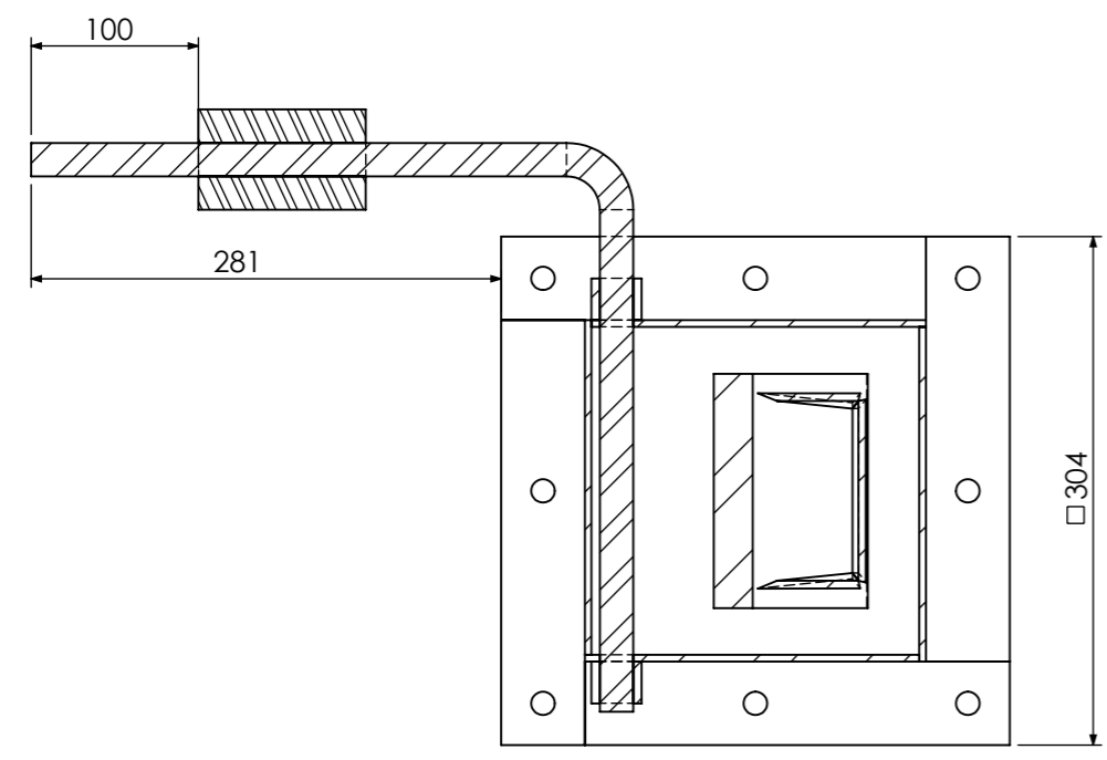
SECTION CG-CG
