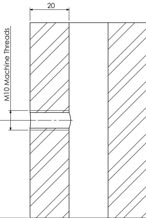
SECTION CK-CK
