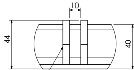
DETAIL AW SCALE 1 : 2
