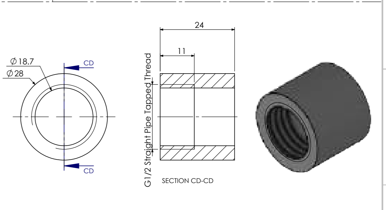
Bag filter pressurized air tank bush.02 BF-01-03-06-01-11
