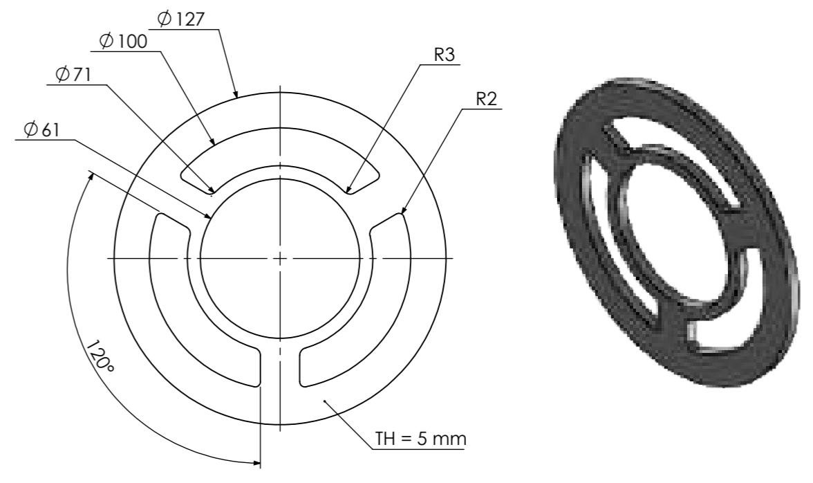
Bag filter pressurized air tank plate.01 BF-01-03-06-01-02
