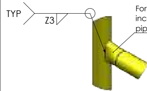
DETAIL AC SCALE 1 : 4
