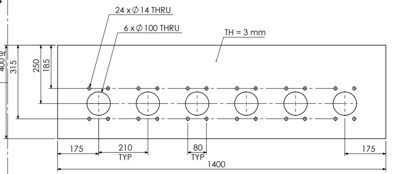
Bag filter clean gas chamber body plate.05 BF-01-03-01-13
