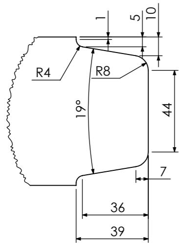
DETAIL N SCALE 1 : 1
