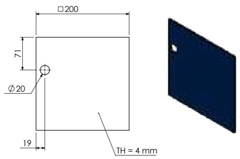
Bag filter air lock welded plate.02 BF-01-04-01-01
