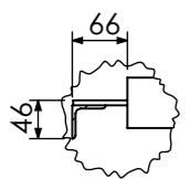
DETAIL AG SCALE 1 : 10
