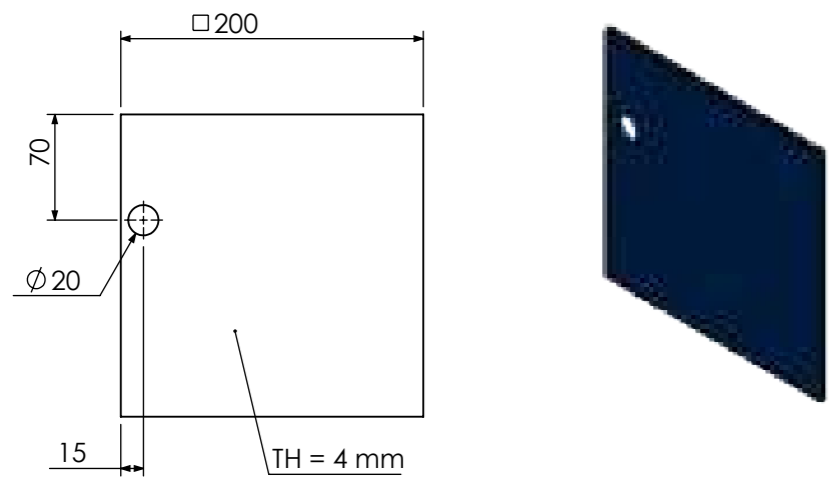
Bag filter air lock welded plate.04 BF-01-04-01-03
