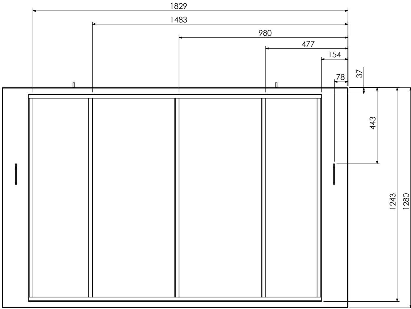
VIEW BH
