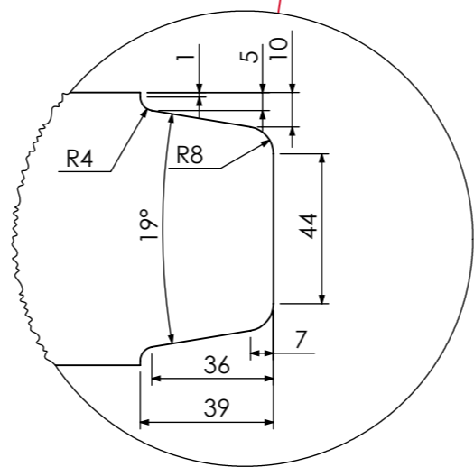
Bag filter walk way UPN80.03 BF-01-01-02-03
