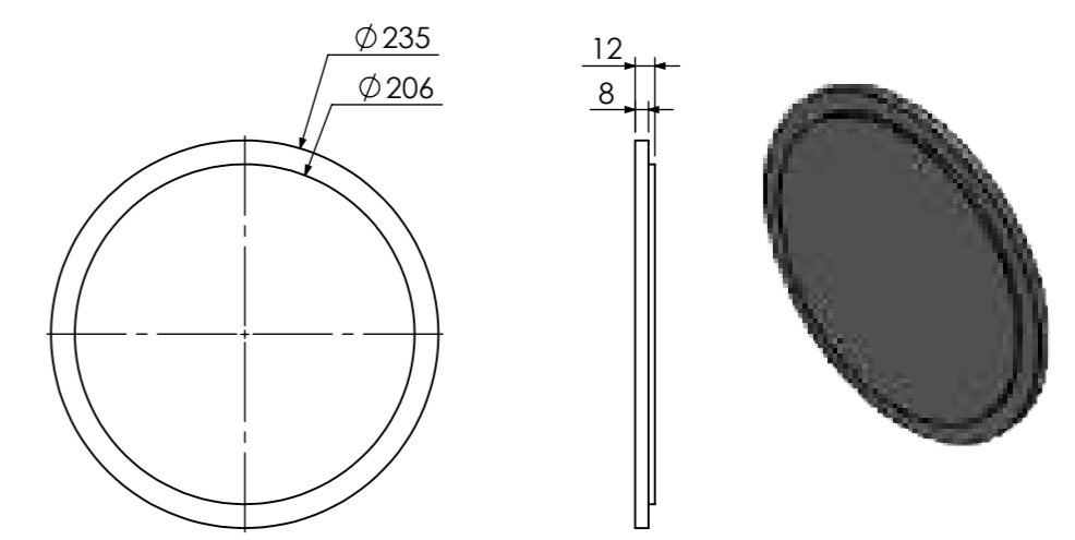
Bag filter pressurized air tank plate.01 BF-01-03-06-01-02
